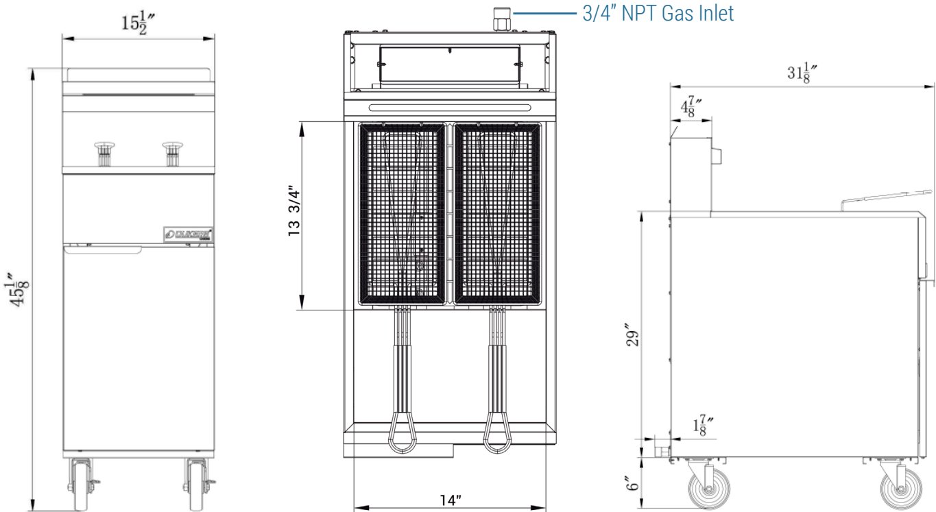
Front View
